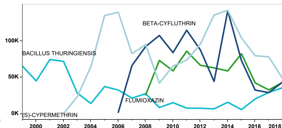
Alfalfa acres treated by the major AIs from 1999 to 2018. The graphs are ordered by the acres treated in 2018 starting with the largest amount in the upper left, moving to the right, then down. The line colors represent the AI type: blue represents insecticides, green herbicides, gray fungicides, red fumigants, insecticide/fungicides yellow, defoliants orange, and others purple. Within each graph, the lines of different AIs of one type have different color intensities
