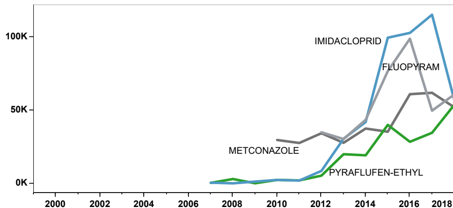
Pistachio acres treated by the major AIs from 1999 to 2018. The graphs are ordered by the acres treated in 2018 starting with the largest amount in the upper left, moving to the right, then down. The line colors represent the AI type: blue represents insecticides, green herbicides, gray fungicides, red fumigants, insecticide/fungicides yellow, defoliants orange, and others purple. Within each graph, the lines of different AIs of one type have different color intensities
